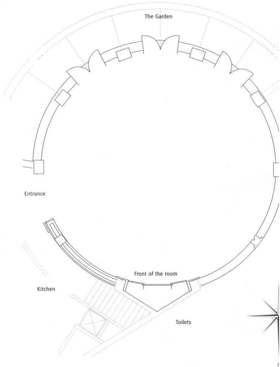
PAVILION FLOOR PLAN
